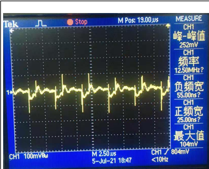
Noise (VIN = 42V, IO = 3A, 5 ~ 20MHz bandwidth)
