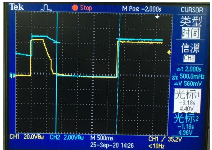
Output response & load (5V / 1.5A)
