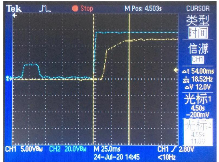
Output response & load (12V / 0.02A)
