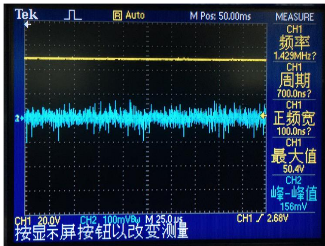
Noise (VIN = 48V, IO = 3A, 5 ~ 20MHz bandwidth)
