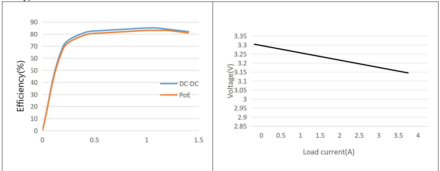
Efficiency ( V_{out} = 3.3 V )
