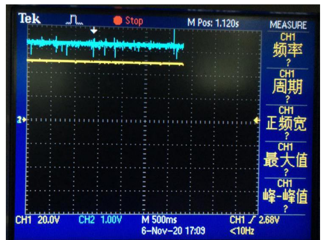
Output response & load (3.3V / 3A)
