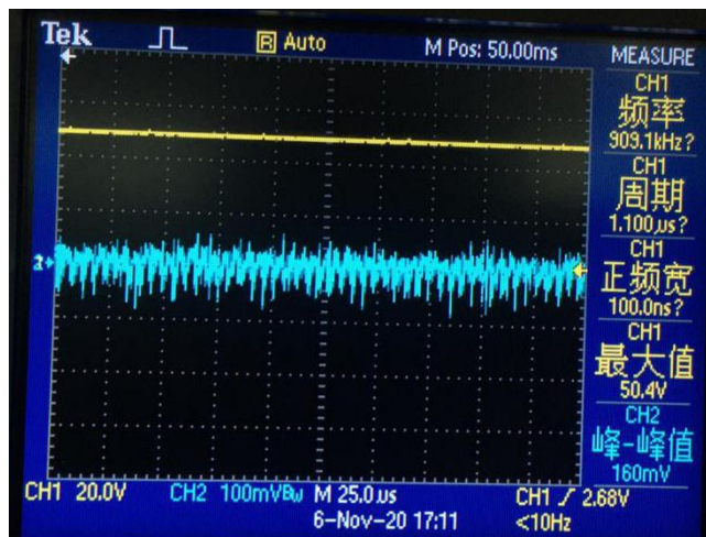
Noise (VIN = 57V, IO = 3A, 5 ~ 20MHz bandwidth)
