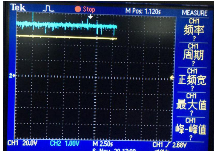
Output response & load (3.3V / 1A)
