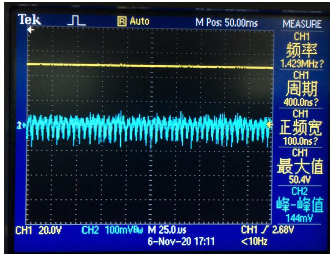
Noise (VIN = 42V, IO = 3A, 5 ~ 20MHz bandwidth)
