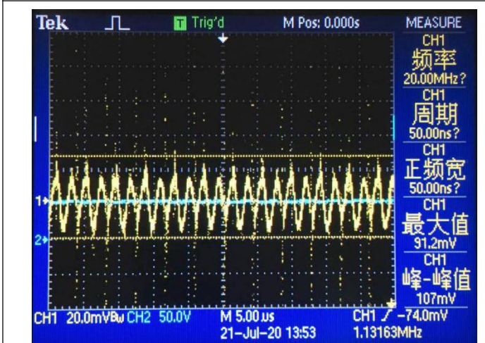
Noise (VIN = 57V, IO = 1A, 5 ~ 20MHz bandwidth)
