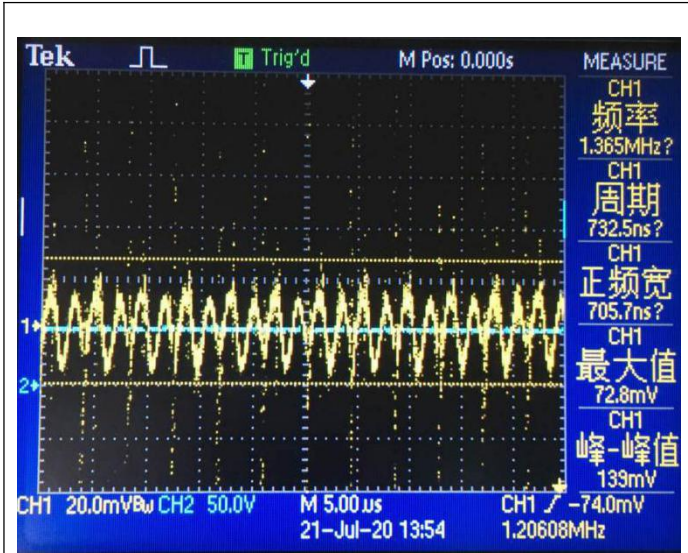
Noise (VIN = 42V, IO = 1A, 5 ~ 20MHz bandwidth)
