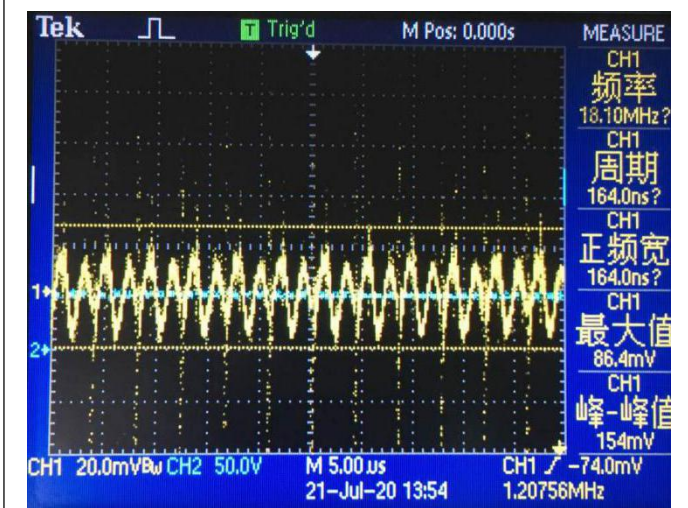
Noise (VIN = 48V, IO = 1A, 5 ~ 20MHz bandwidth)
