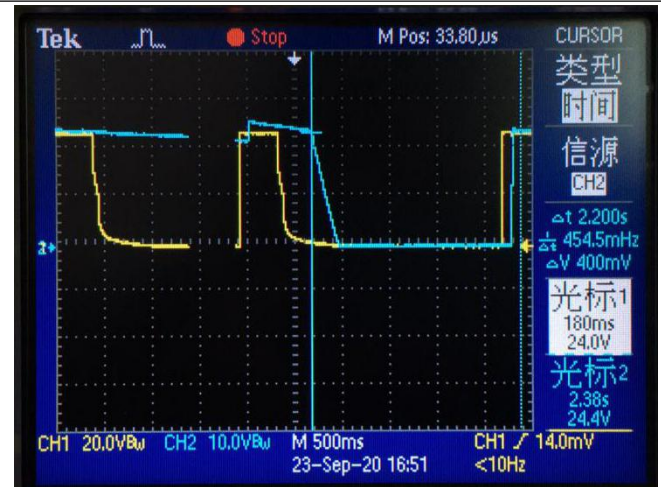
Output response & load (24V / 1A)
