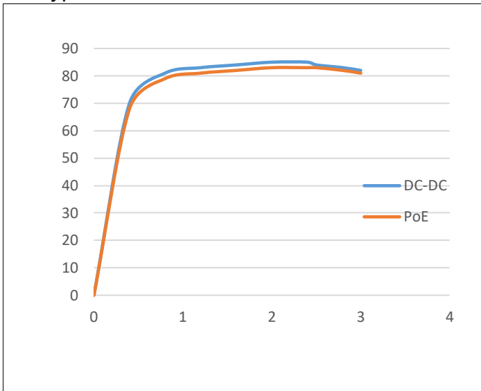
Efficiency (Vout = 12 V)
