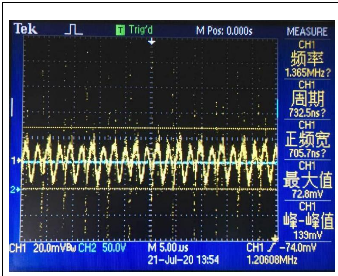
Noise (VIN = 42V, IO = 2A, 5 ~ 20MHz bandwidth)
