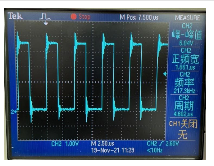
PWM waveform
