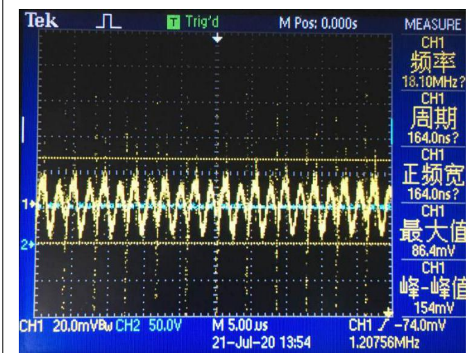
Noise (VIN = 48V, IO = 6A, 5 ~ 20MHz bandwidth)
