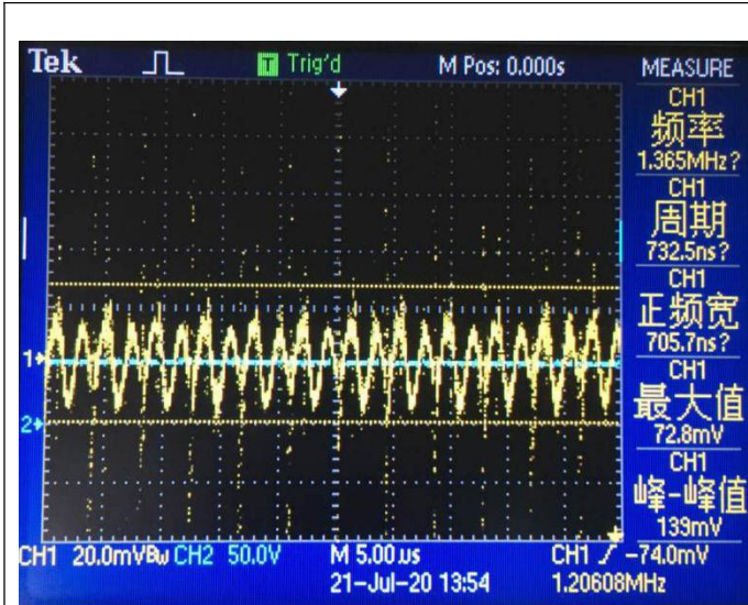
Noise (VIN = 42V, IO = 6A, 5 ~ 20MHz bandwidth)
