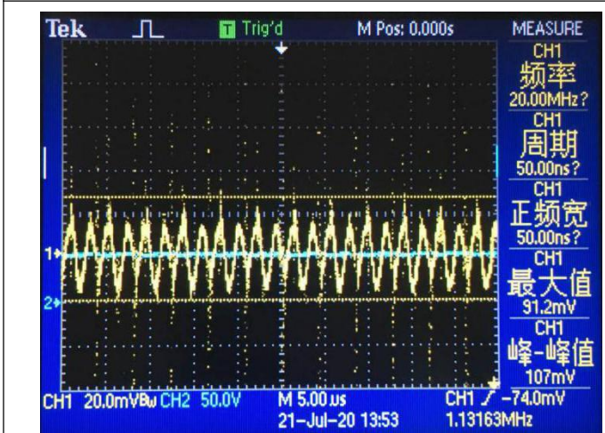
Noise (VIN = 57V, IO = 6A, 5 ~ 20MHz bandwidth)
