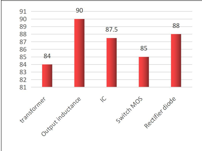
Maximum temperature of components Conditions (ambient temperature: 27 °C; output power: 5V / 6A; frequency: 3H)
