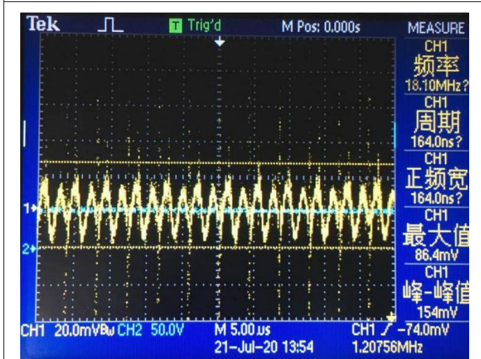
Noise (VIN = 42V, IO = 2.5A, 5 ~ 20MHz bandwidth)
